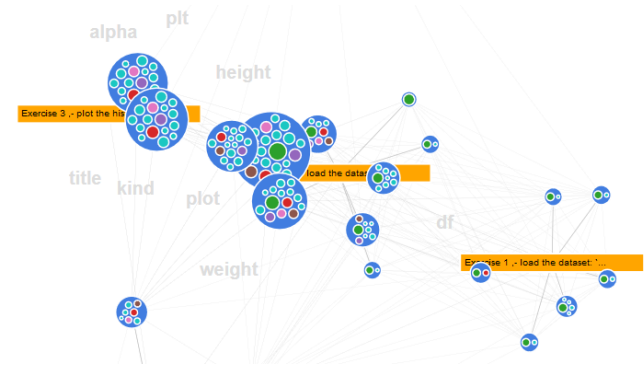
Figure 4: Cell nodes include the collection of common variables, functions, and string literals used in the corresponding code cell. The frequency of each component within the full notebook is indicated using both area and color.
